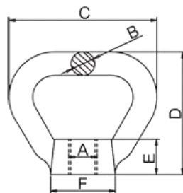
Triangle Eye Bolt
